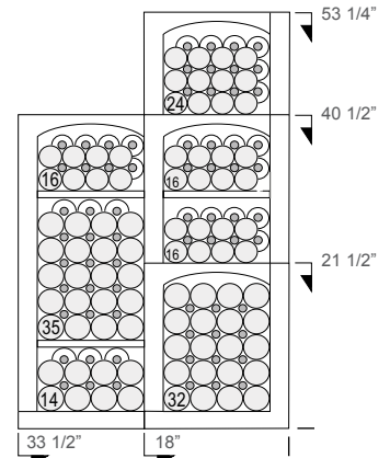
1 view/dimensions in inches
